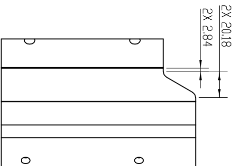
VIEW B-B
